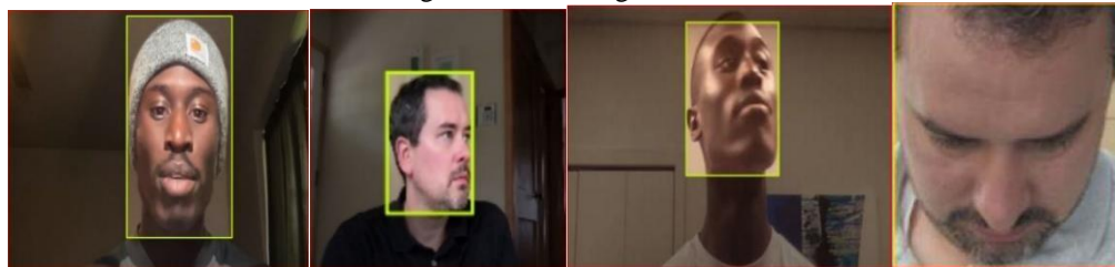
Fig 4: Dataset Images
