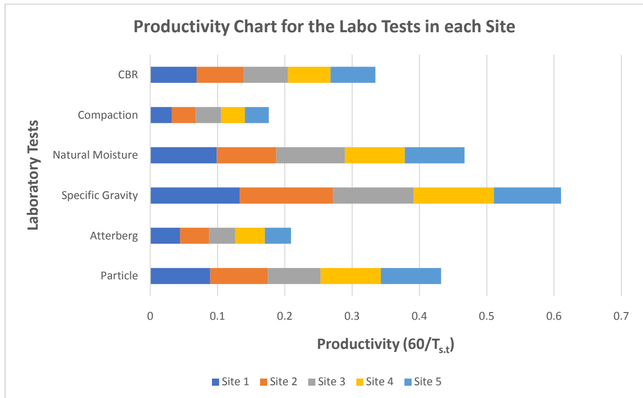
Fig 3.2: Chart showing The productivity of each Site on the different laboratory tests
