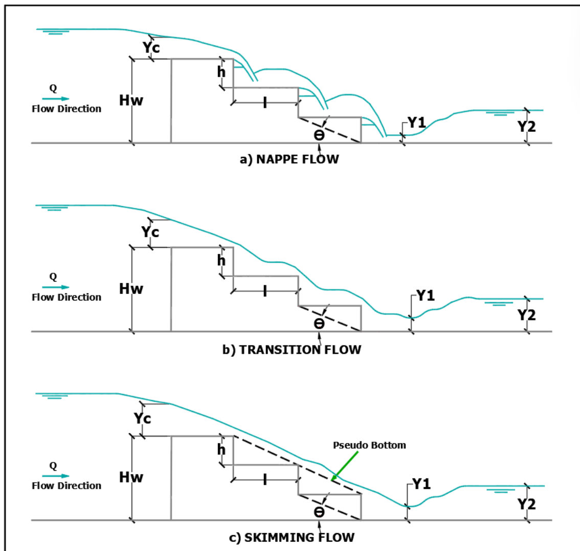
Figure 5: The different flow regimes of stepped chutes (a) nappe flow regime, (b) transition flow regime, and (c) skimming flow regime (Adapted from (Salmasi and Özger 2014)).
