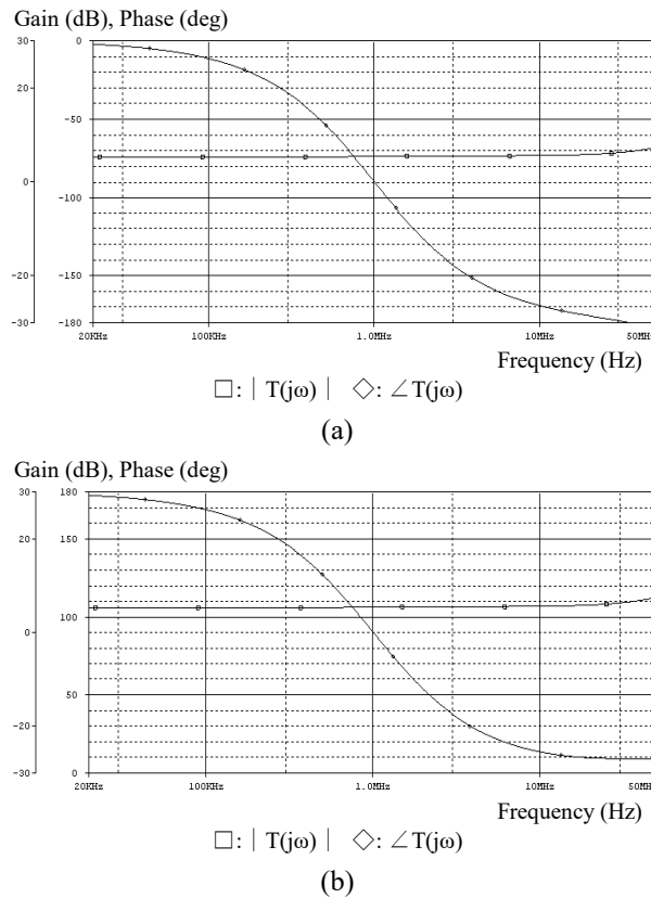
Figure 5: Voltage-mode simulation responses ((a) plus current output, (b) minus current output)
