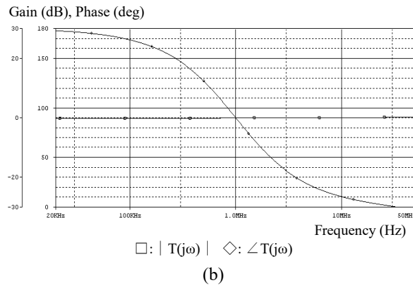
Figure 8: Current-mode simulation responses ((a) plus current output, (b) minus current output)
