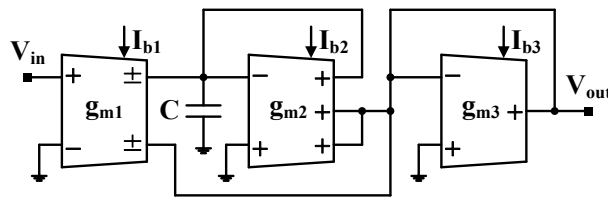
Figure 3: Voltage-mode APS configuration
