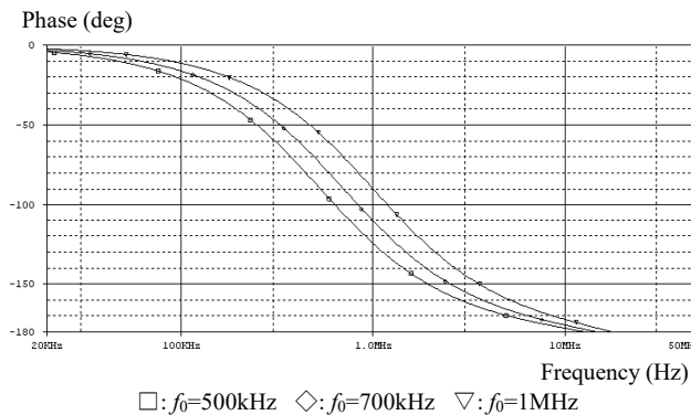
Figure 10: Current-mode f_0 -tuning responses
