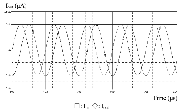
Figure 9: Current-mode input and output waveforms
