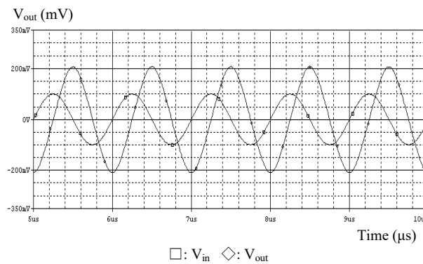
Figure 7: Voltage-mode input and output waveforms
