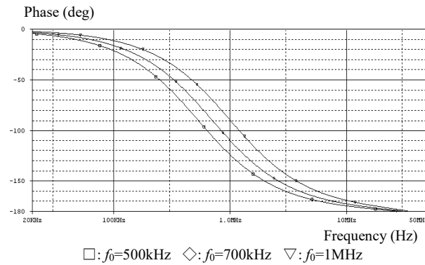
Figure 6.: Voltage-mode f_0 -tuning responses
