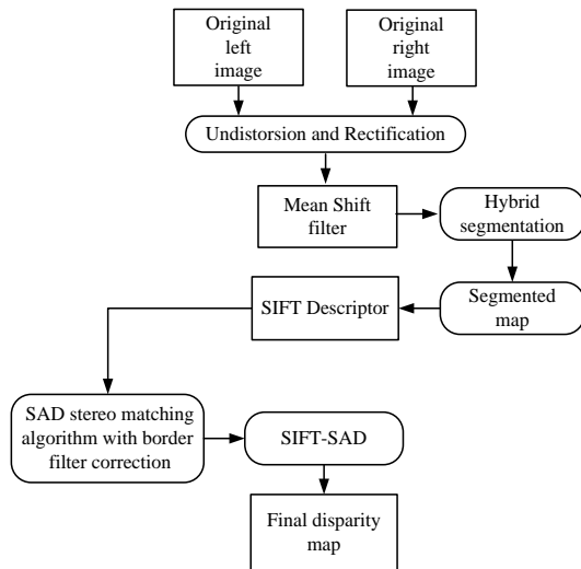
Fig. 3. Block diagram of proposed approach using SIFT-SAD algorithm
