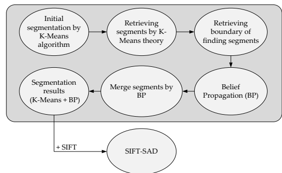
Fig. 2. Hybrid segmentation algorithm
