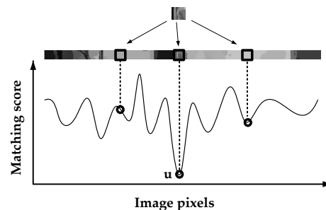
Fig. 5. Best matching pixel (minimum value over the row)
