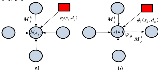
Fig. 1. (a) Computing belief, (b) Computing message [4]
