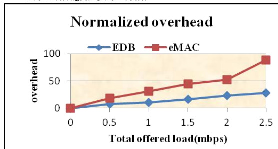
Fig.6. Total offered load Vs Overhead.
