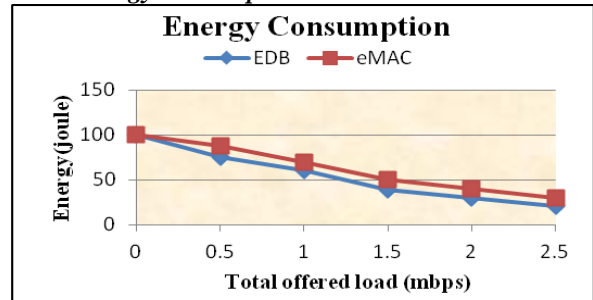
Fig.8. Performance of energy consumption across various loads.
