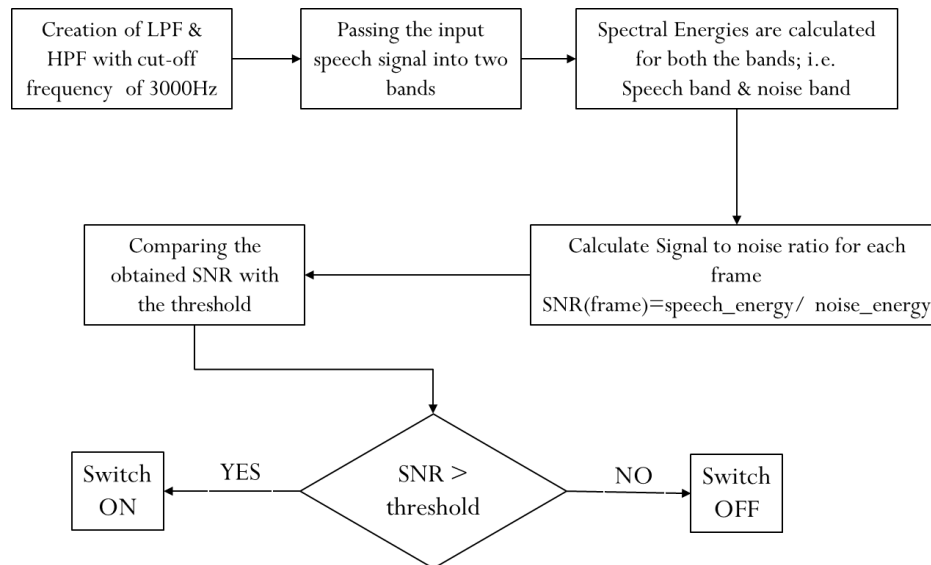
Fig2 : Conventional energy based algorithm - flowchart
