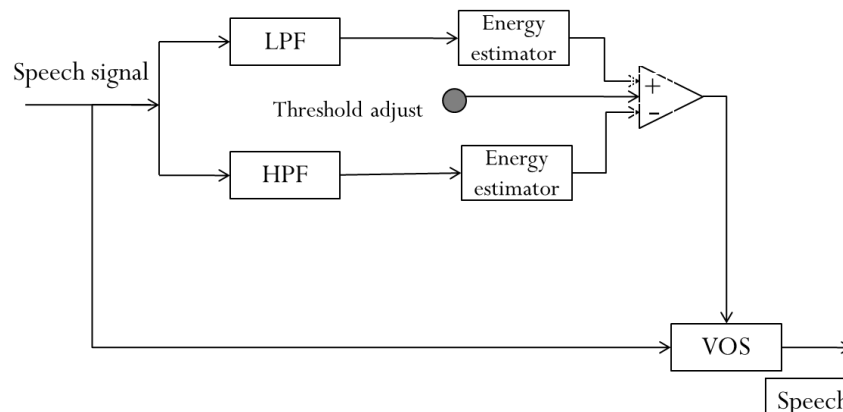
Fig1: Conventional energy based algorithm block diagram
