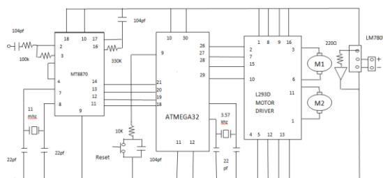
Fig2:circuit diagram of mobile operated land rover
