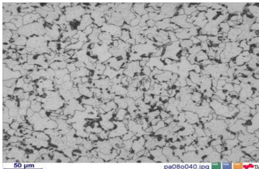
Figure 1. Microstructure of virgin steam line material 14MoV6-3, magnification 200x, [6]
