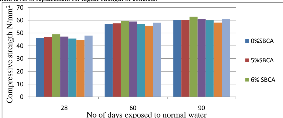
GRAPH.1: Compressive strength results of SBCA Concrete cured in normal Water
