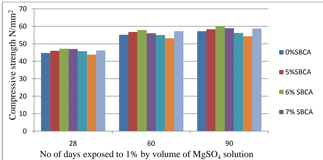
GRAPH.5: Compressive strength results of SBCA Concrete exposed to 1% by volume of MgSO_4 solution
