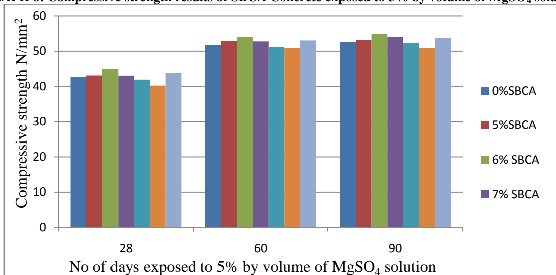
GRAPH 7: Compressive strength results of SBCA Concrete exposed to 5% by volume of MgSO_4 solution.
