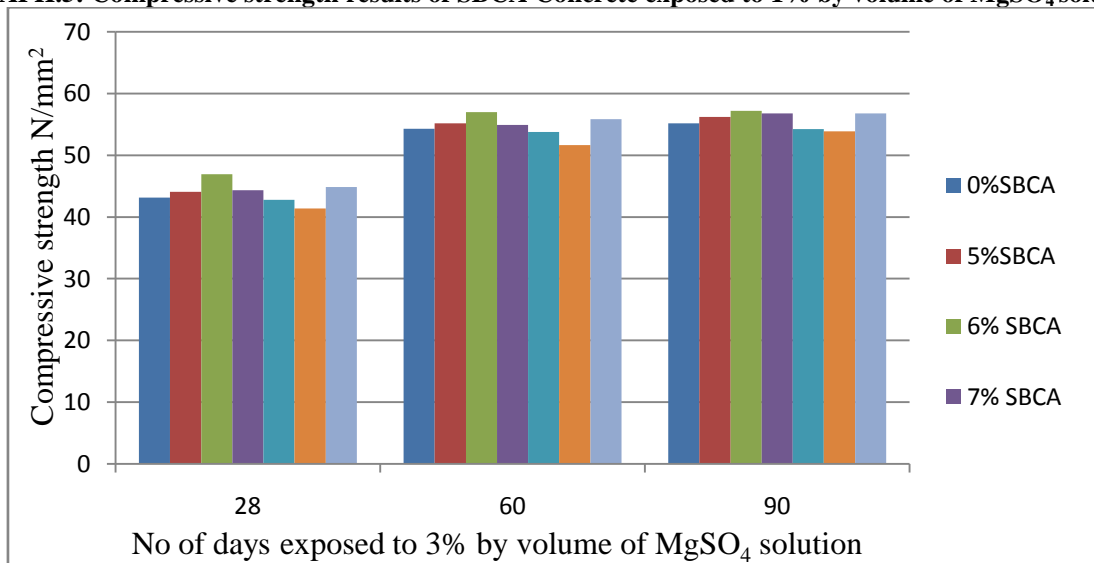
GRAPH 6: Compressive strength results of SBCA Concrete exposed to 3% by volume of MgSO_4 solution.
