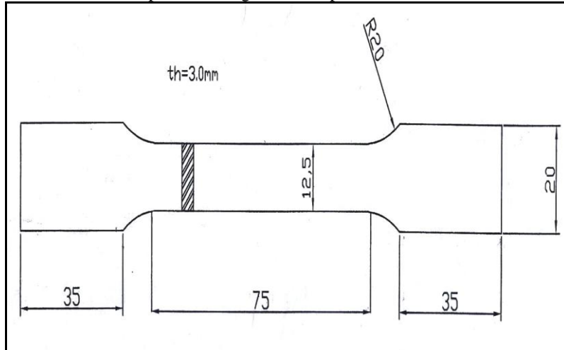
Figure (3) Show the dimension of tensile specimens Din50120
