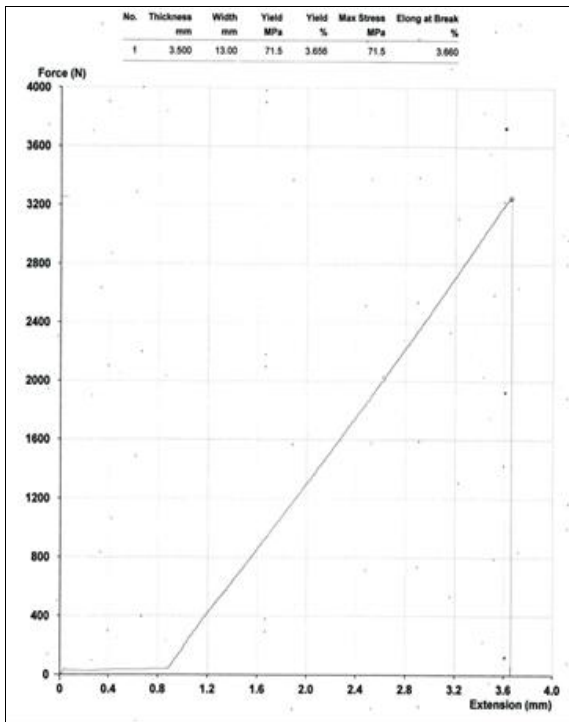
Figure (7) diagram: specimen No.4
