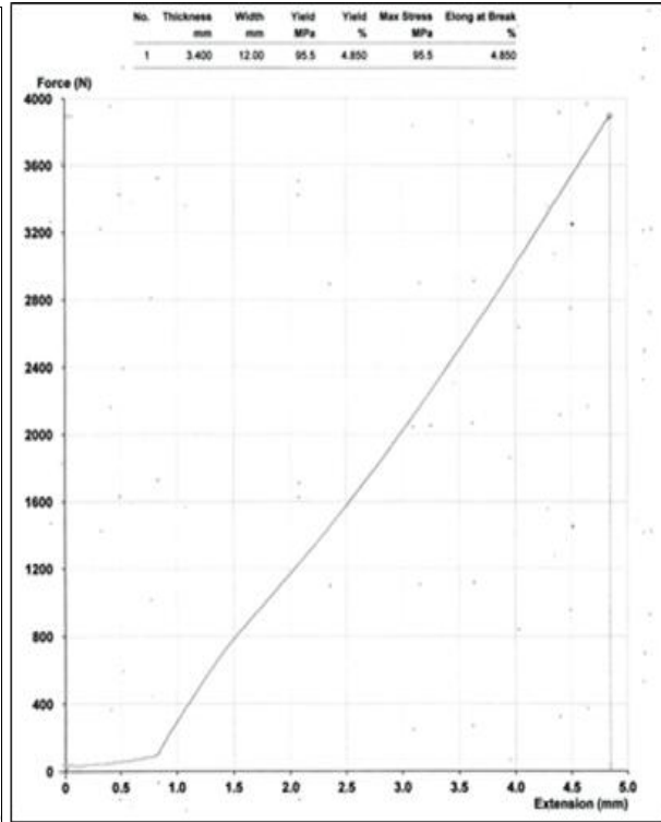
Figure (6) diagram: specimen No.3
