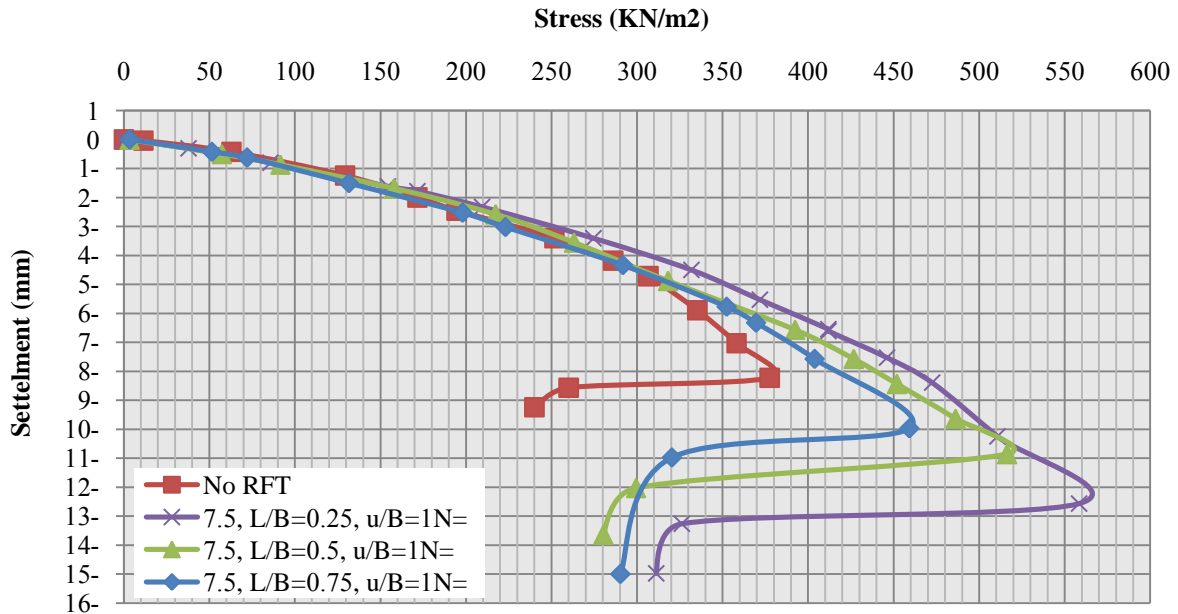
Figure 21: Variation of u/B with footing (C) Experimental Results
