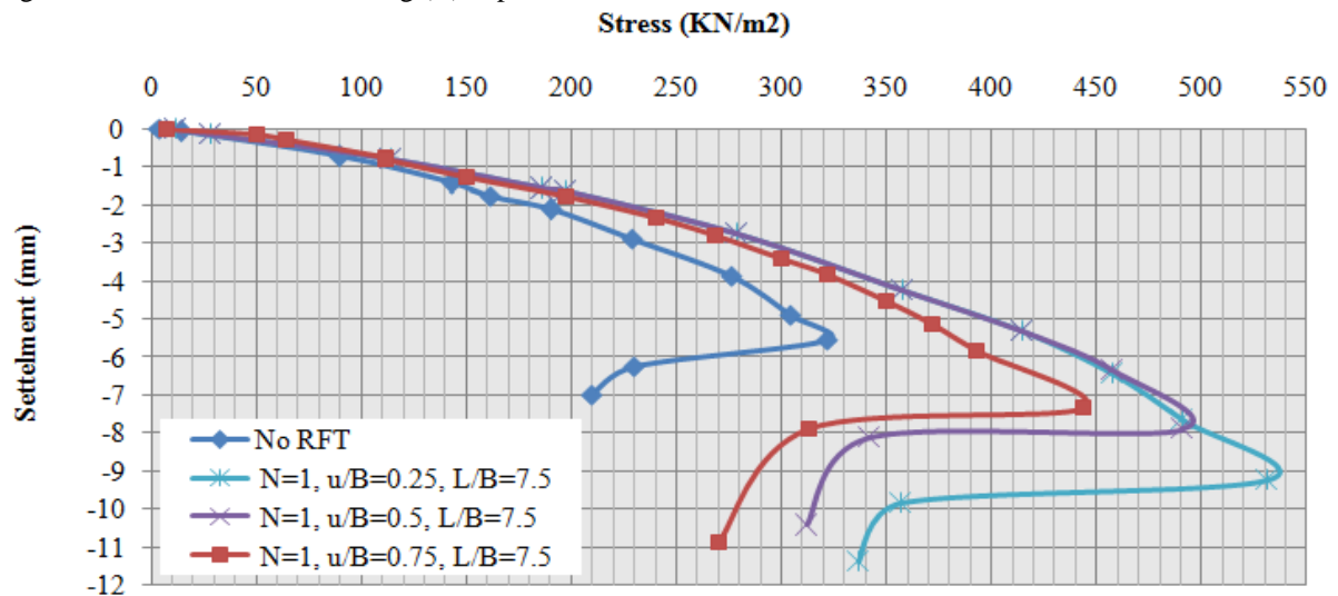
Figure 20: Variation of u/B with footing (B) Experimental Results
