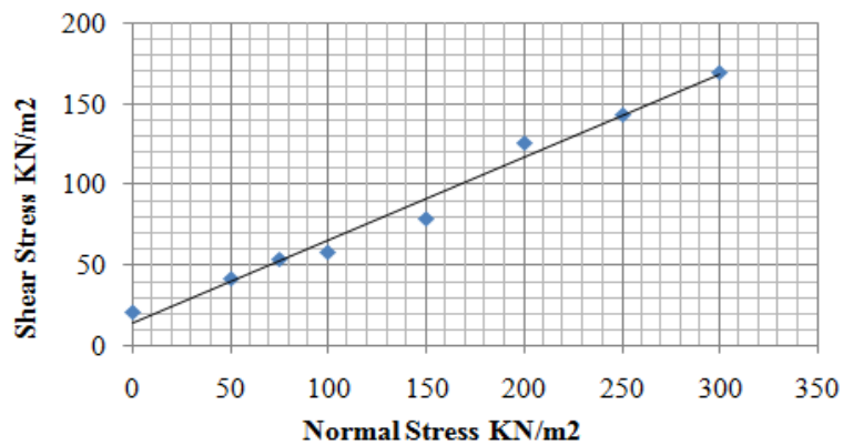
Figure 2: Direct Shear Test Result
