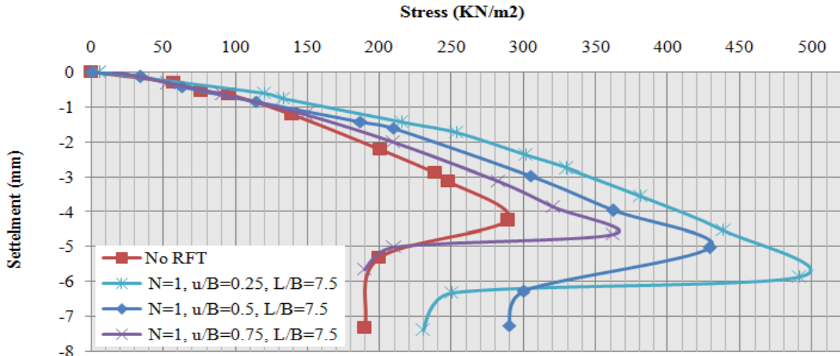
Figure19: Variation of u/B with footing (A) Experimental Results
