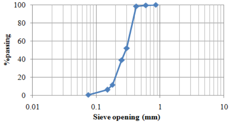
Figure 1: Sieve Analysis results
