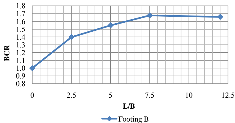
Figure 24: BCR vs. L/B for footing (B)
