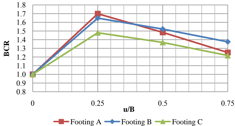
Figure 23: BCR vs. u/B for footing (A), (B) & (C)
