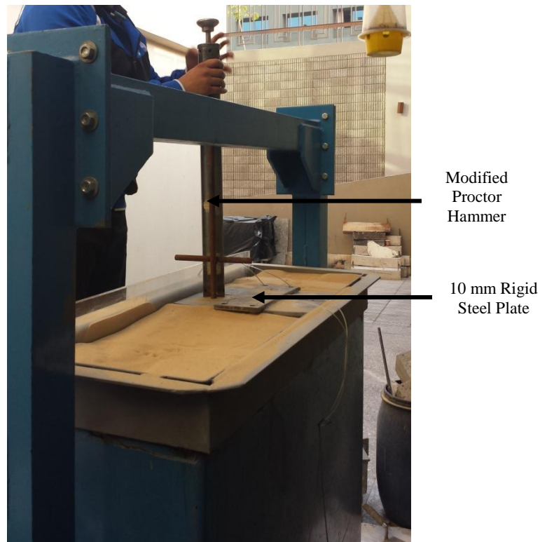
Figure 14: Preparation of sand bed
