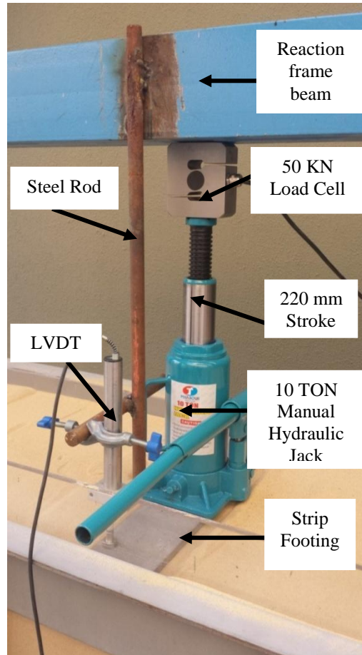
Figure12: The loading system with measuring instruments
