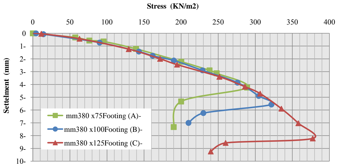
Figure 18: Unreinforced Soil bed Experimental results
