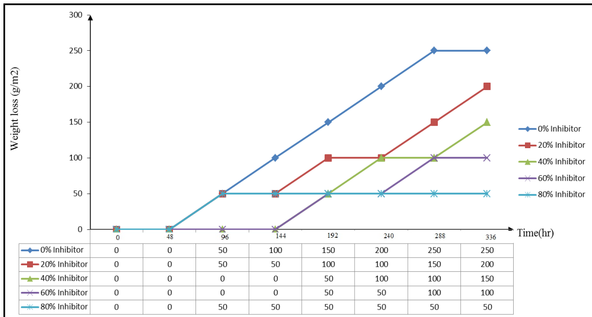
Figure 1: Weight loss-time curves of carbon steel in 0.1M HCl in the absence and presence of different concentrations of Cashew inhibitor.
