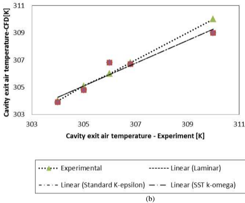
Fig.3 Comparison between CFD results and experimental data from the literature for flat UTC model: (a) plate surface temperature and (b) cavity exit air temperature.
