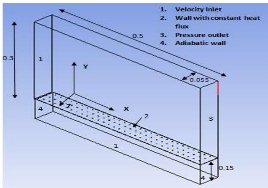
Fig.1 (a) Flat UTC model configuration (unit: m) – Computational Domain
