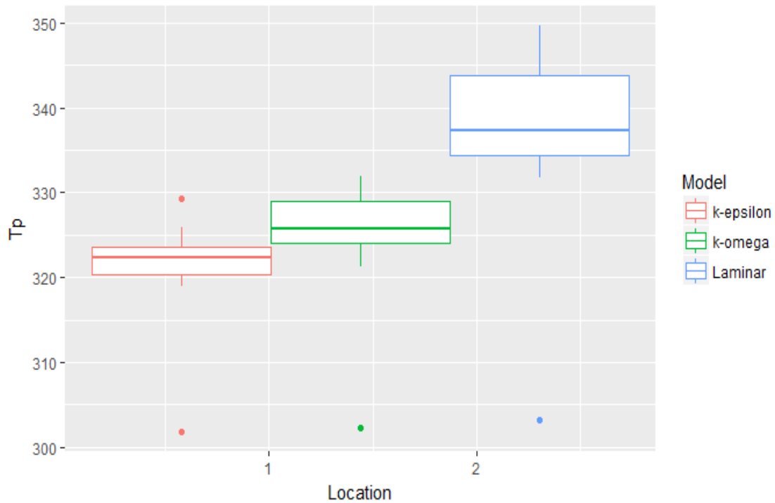
Fig.7 Box plots to show the range and characteristics of plate temperatures predicted by 3 different models k- \omega (k-omega), Laminar and k- \epsilon (k-epsilon) for suction velocity, V_s = 0.077 m/s
