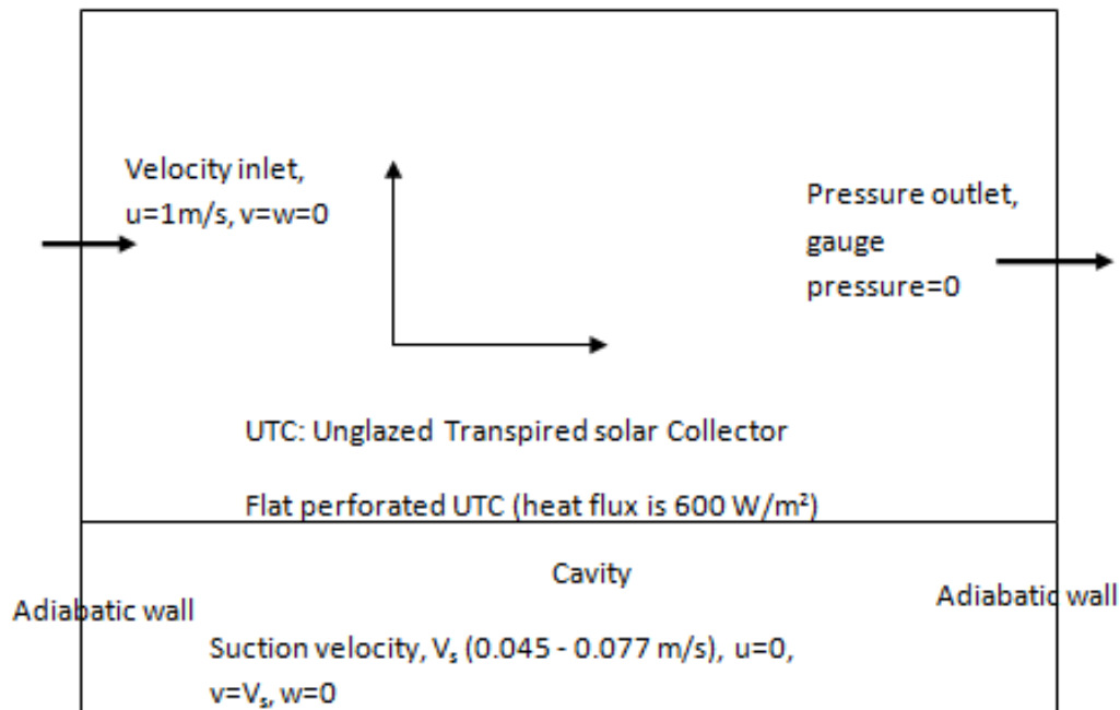
Fig.2 Schematic diagram with boundary condition for the flow domain in X-Y plane
