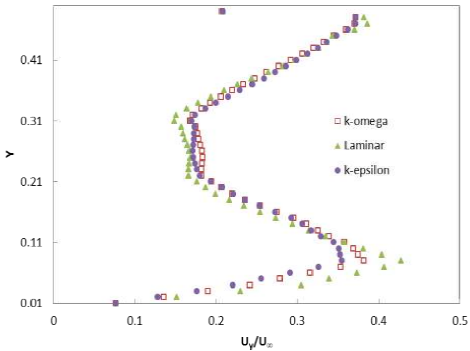
Fig.5 Comparison of velocity profile, U_y of hot air within the chamber predicted by 3 different models k- \omega , Laminar and k- \epsilon for suction velocity, V_s= 0.077 m/s
